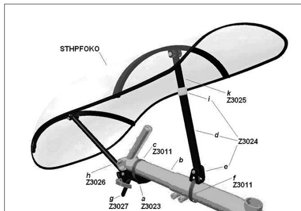
The unique Quickmount system attaches easily to the bike's frame.
